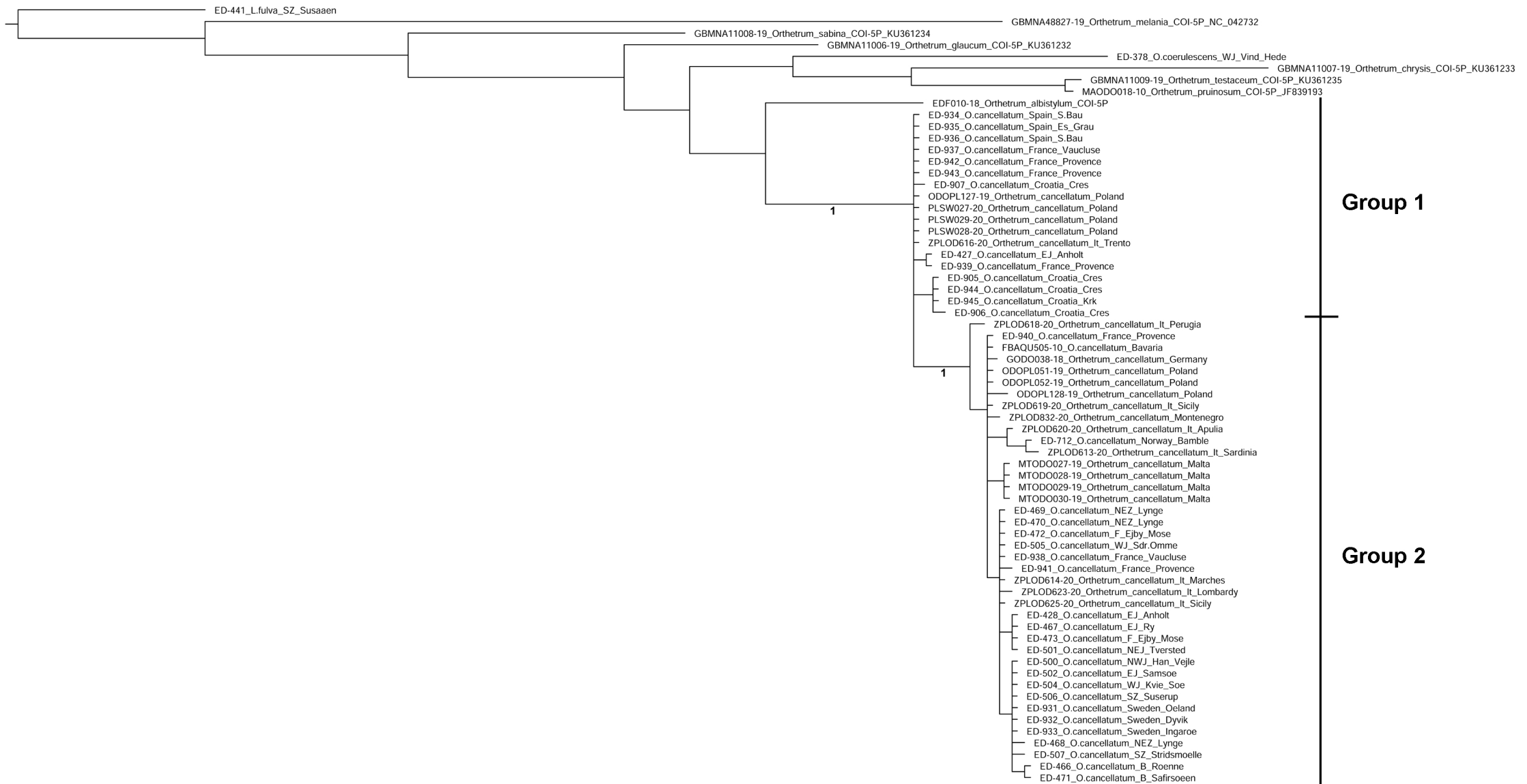
Supplementary matrial S2. Tree from the 10 million generation analysis of the Orthetrum cancellatum COI barcode dataset in MrBayes. Numbers indicate relavant posterior probability values above 0.9.
